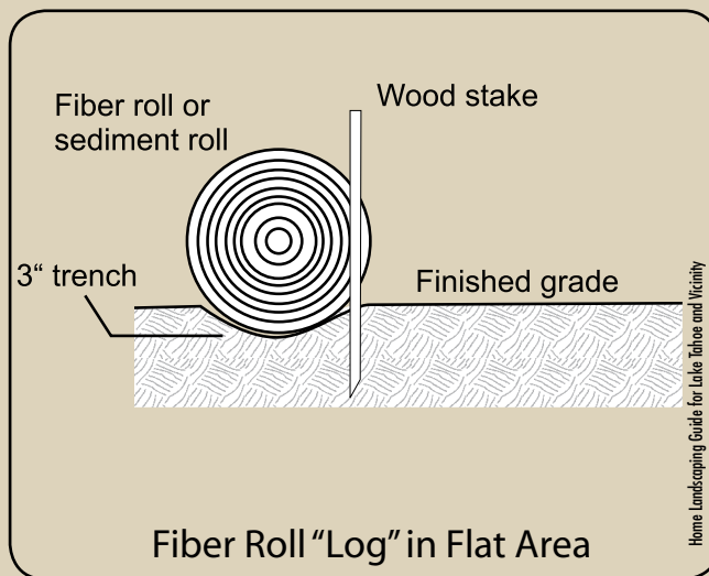
Temporary Erosion Control. Filter fences and fiber roll sediment barriers help guard against erosion during construction or soil moving activities.
